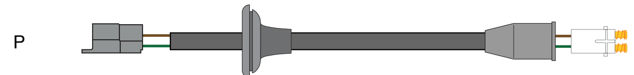
(Right Hand Tail Light Boot Assy - Reference, 1 pc.)
