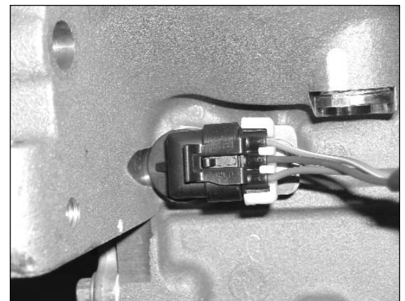
Figure 5 - Crankshaft Position Sensor
