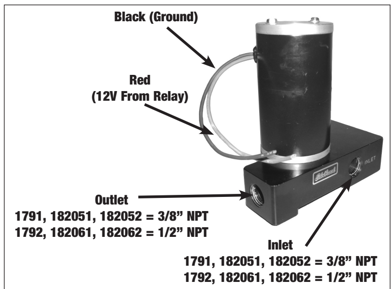
Figure 2 - Fuel Pump
