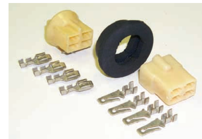
firewall disconnects (4,6,8, & 9 wire applications)
